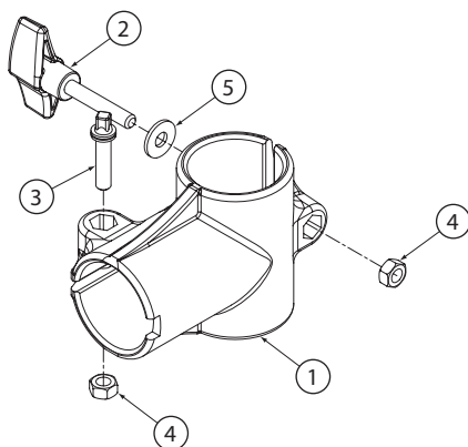
Exploded View (Fig.3)
