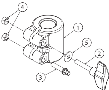
Exploded View (Fig.2)
