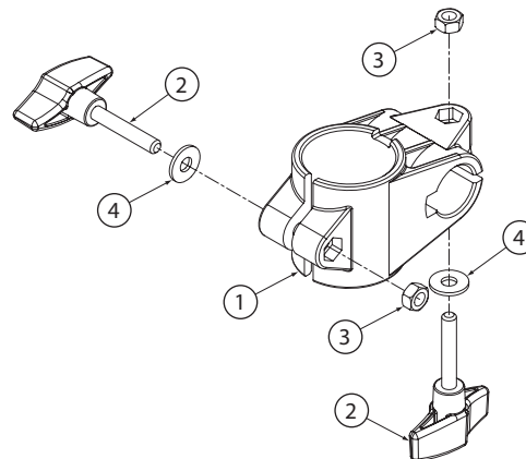
Exploded View (Fig.5)
