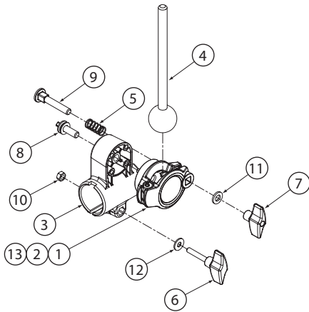
Exploded View (Fig.1)
