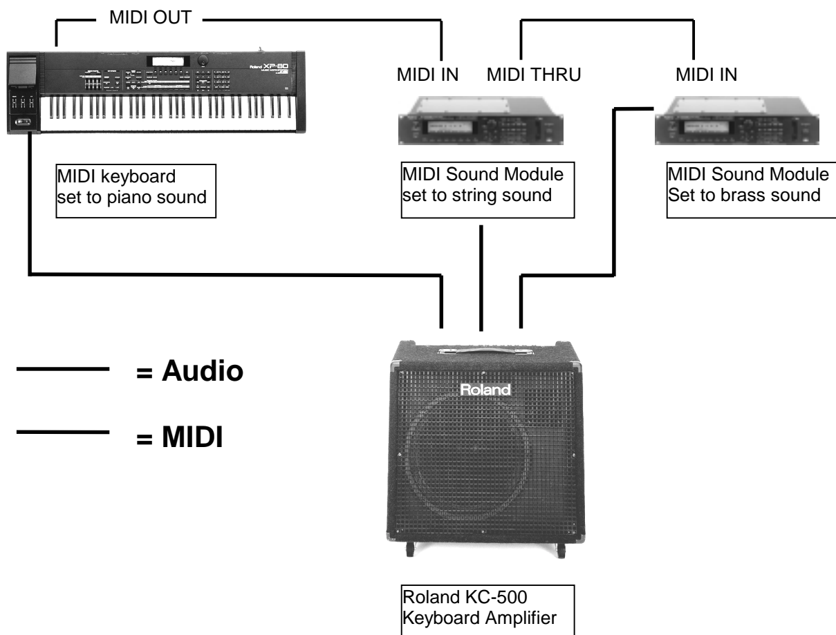
Fig. 3 MIDI and Audio Connections
